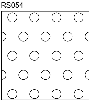
Hole Size: 5/32" Dia. x 3/8" Ctrs. Open Percentage: 16%
