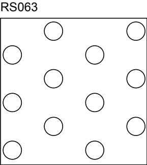
Hole Size: 3/16" Dia. x .487" Ctrs. Open Percentage: 13%
