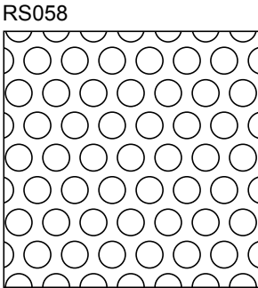
Hole Size: 5/32" Dia. x 7/32" Ctrs. Open Percentage: 46%
