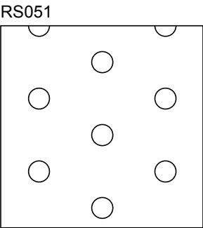
Hole Size: 5/32" Dia. x .541" Ctrs. Open Percentage: 8%
