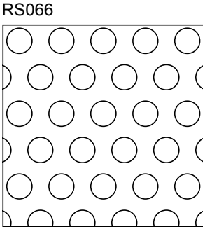
Hole Size: 3/16" Dia. x 5/16" Ctrs. Open Percentage: 33%
