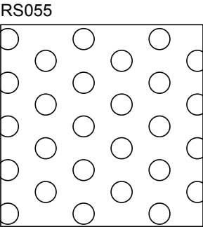
Hole Size: 5/32" Dia. x .325" Ctrs. Open Percentage: 21%
