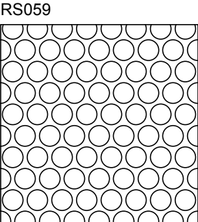
Hole Size: 5/32" Dia. x 3/16" Ctrs. Open Percentage: 62%
