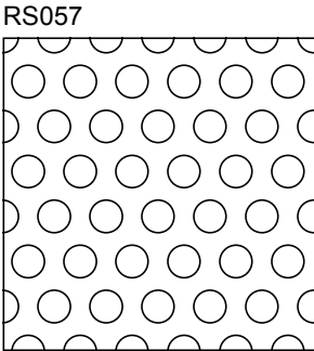
Hole Size: 5/32" Dia. x 1/4" Ctrs. Open Percentage: 35%
