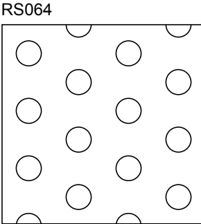
Hole Size: 3/16" Dia. x .433" Ctrs. Open Percentage: 17%
