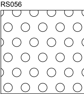
Hole Size: 5/32" Dia. x 5/16" Ctrs. Open Percentage: 23%
