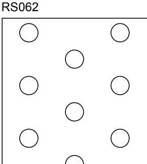
Hole Size: 3/16" Dia. x .541" Ctrs. Open Percentage: 11%
