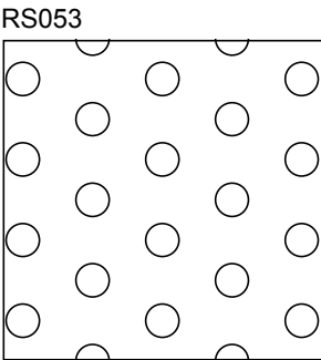
Hole Size: 5/32" Dia. x .379" Ctrs. Open Percentage: 15%
