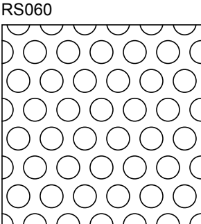
Hole Size: 11/64" Dia. x 1/4" Ctrs. Open Percentage: 43%
