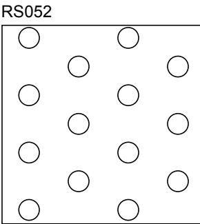
Hole Size: 5/32" Dia. x .433" Ctrs. Open Percentage: 12%
